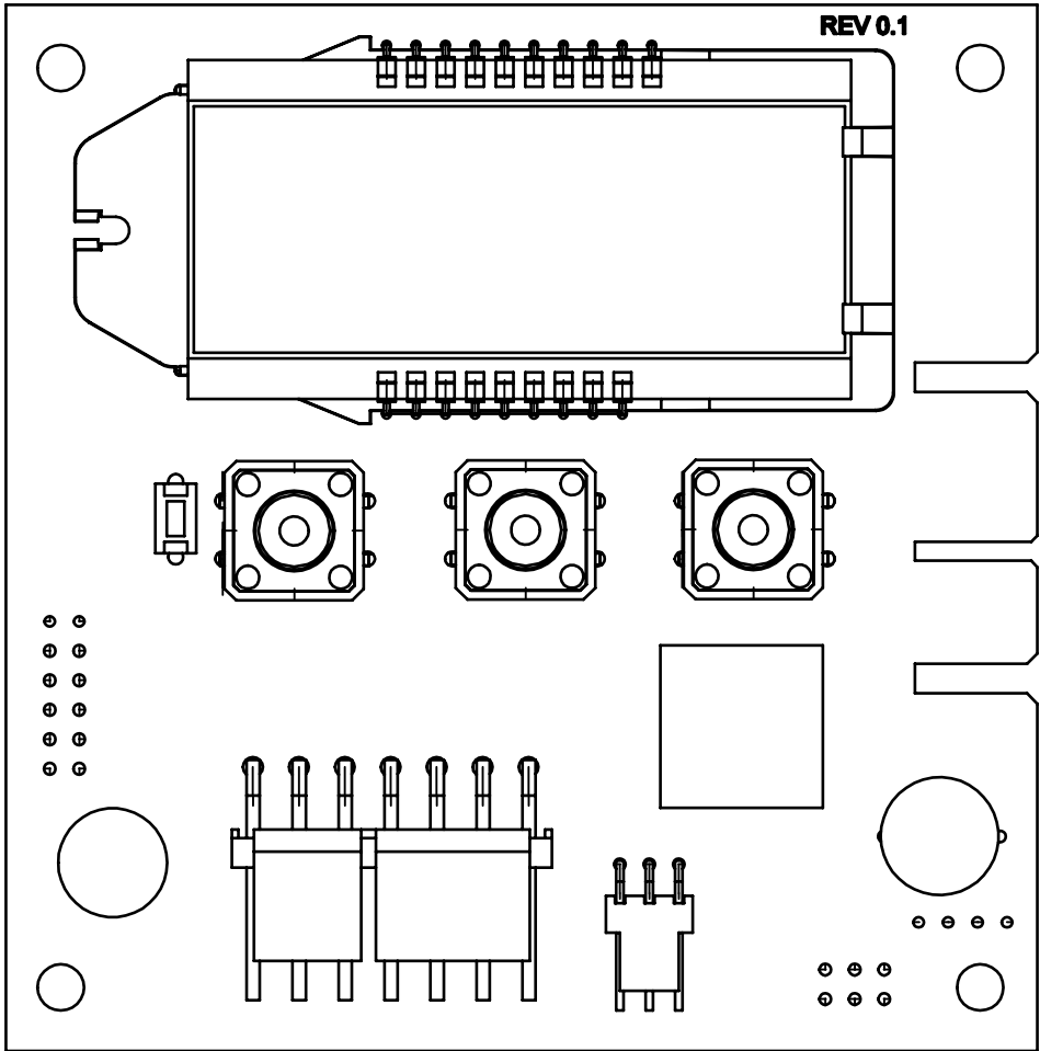
P2 POWER HARNESS
